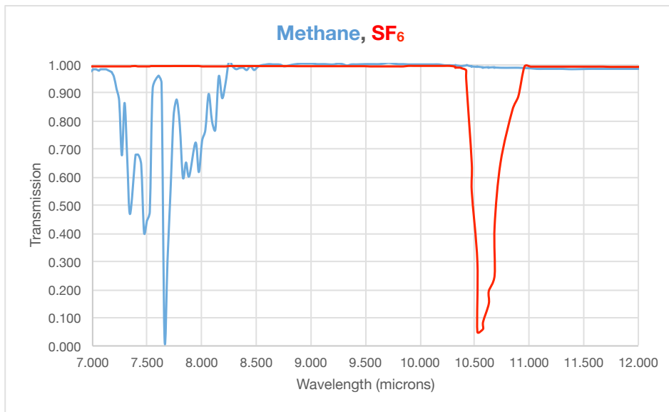
Figure 3: Methane has an absorption spectrum between 7 and 8.5 \mu\text{m} while sulfur hexafluoride's is between 10.5 and 11 \mu\text{m} . (Source: NIST Mass Spec Data Center)
