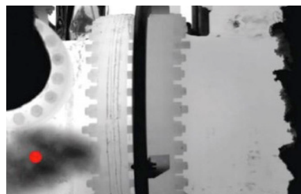
Figure 1: A leak in a natural gas compressor is easily visible using optical gas imaging.
