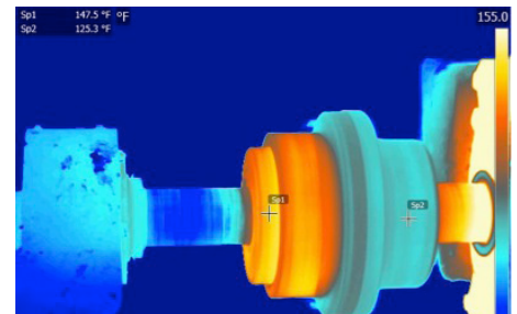
Figure 4: IR imaging can spot temperature differences that indicate equipment failure.
